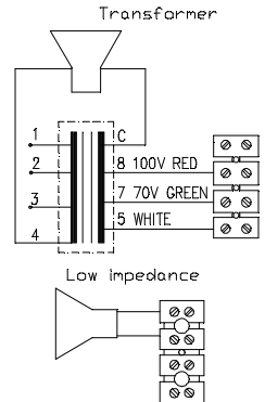
CIRCUIT DIAGRAM
