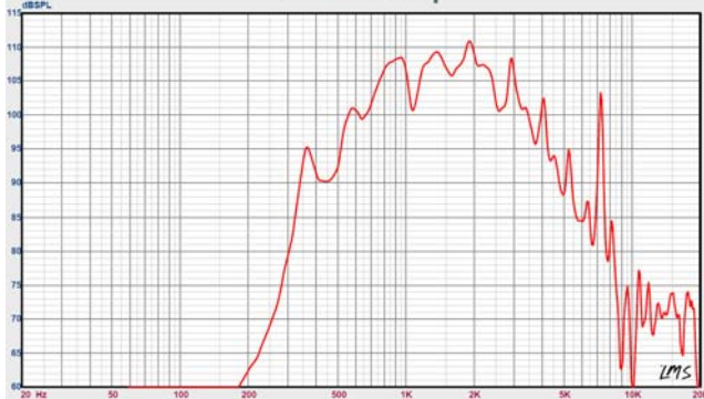
Sound pressure levels at 1W/1m Ferit SPL vs Freq
